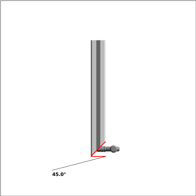
DRAWING 7, Pos 16 SIDE 1, bar length: 235.1 mm
