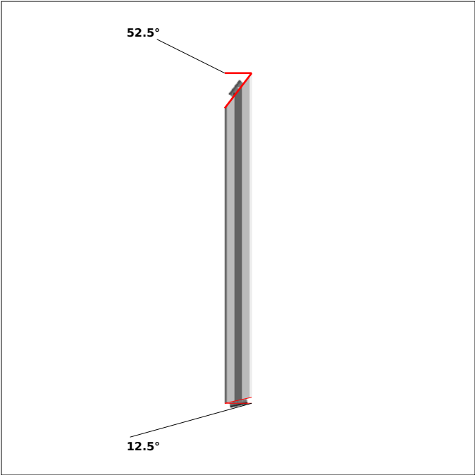
DRAWING 3, Pos 6 SIDE 1, bar length: 368.3 mm
