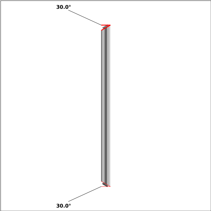
DRAWING 12, Pos 21 SIDE 1, bar length: 527.7 mm
