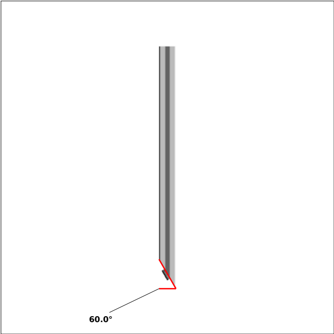
DRAWING 9, Pos 18 SIDE 1, bar length: 428.0 mm
