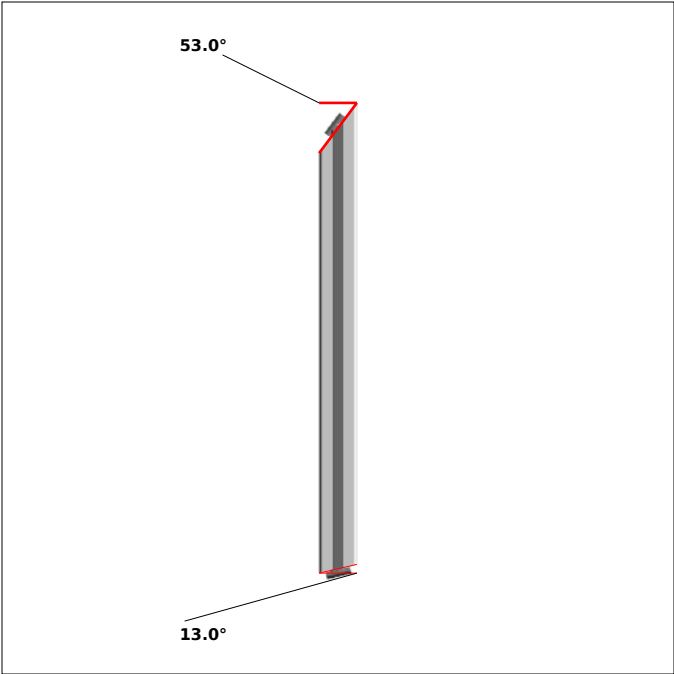
DRAWING 6, Pos 9 SIDE 1, bar length: 372.8 mm
