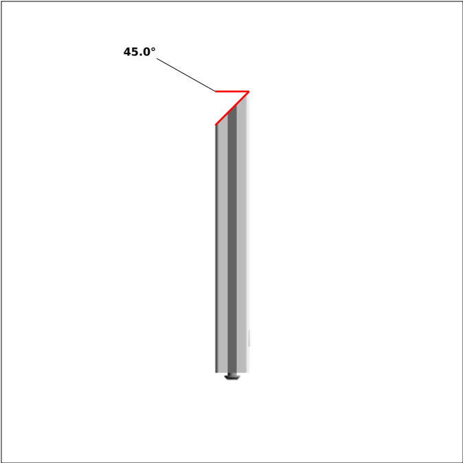
DRAWING 8, Pos 17 SIDE 1, bar length: 250.0 mm
