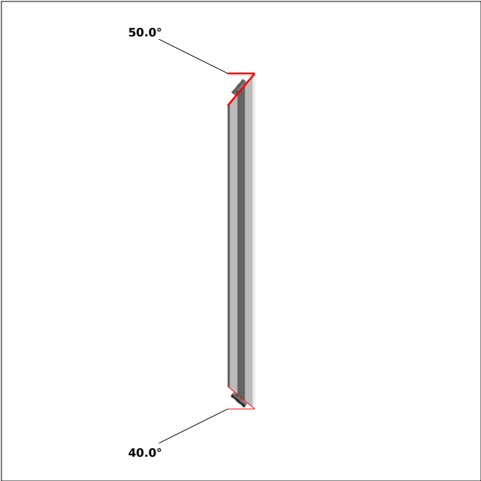
DRAWING 4, Pos 7 SIDE 1, bar length: 372.7 mm
