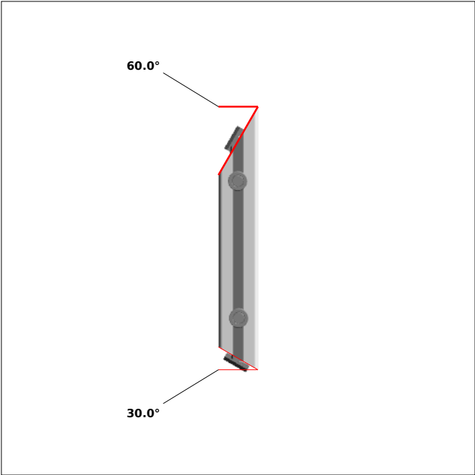
DRAWING 2, Pos 3 SIDE 1, bar length: 200.0 mm
