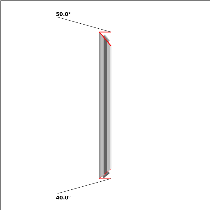
DRAWING 5, Pos 8 SIDE 1, bar length: 372.7 mm
