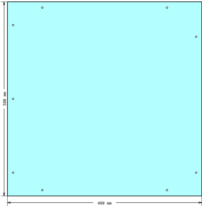
DRAWING 14, Pos 27 Shape measurements
