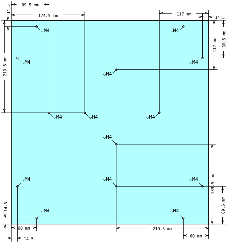
DRAWING 13, Pos 26 Hole placement
