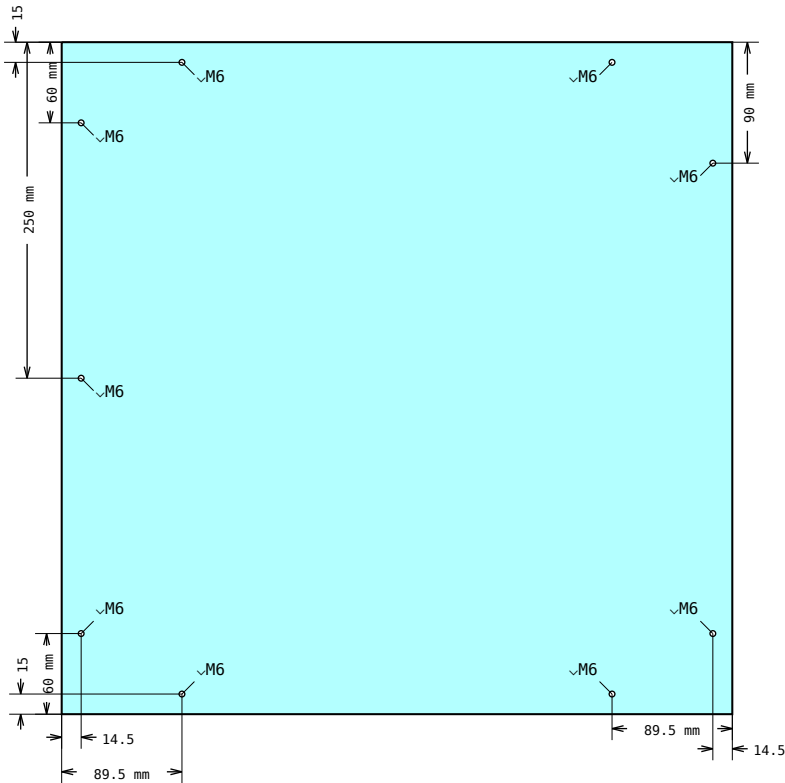
DRAWING 14, Pos 27 Hole placement
