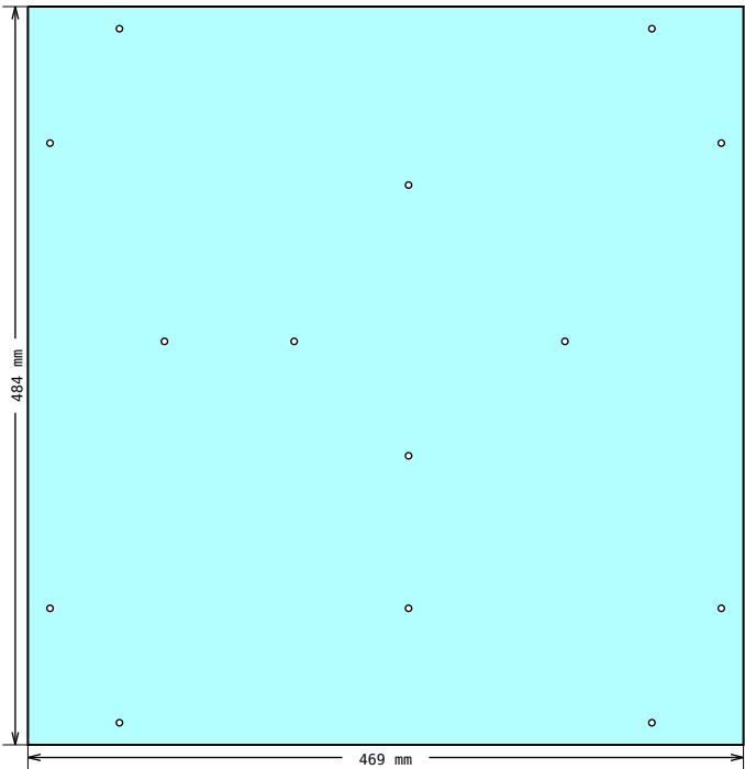
DRAWING 13, Pos 26 Shape measurements
